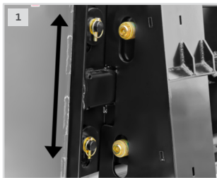
2. DESIGNED TO AUTOMATICALLY KEEP PUSHER WEIGHT ON EDGE FOR CONSISTENT CLEAN-UP & LESS MAINTENANCE
